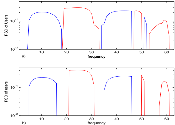
Fig. 1. Optimal PSD at NE in the absence of ICI (subplot a)) and in the presence of ICI (subplot b)) due to frequency offset \Delta f_{r,q} = 0.5/N ; \gamma = 2.5 , d_{12} = d_{21} , d_{11} = d_{22} = 1 , P_1 = P_2 , P_1/\sigma_w^2 = 3 dB, P_1/(\sigma_w^2 d_{12}^2) = 1 dB.
